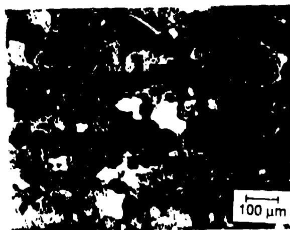
Figure 4 Micrograph of 3.2 mm thick ingot sheet beryllium
