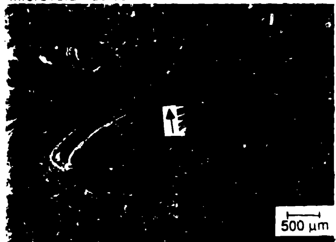
Figure 6. Micrograph displaying centerline crack in ingot sheet beryllium.
