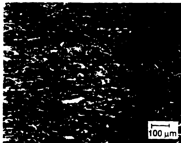
Figure 3. Micrograph of 3.2 mm thick SR200E beryllium.
